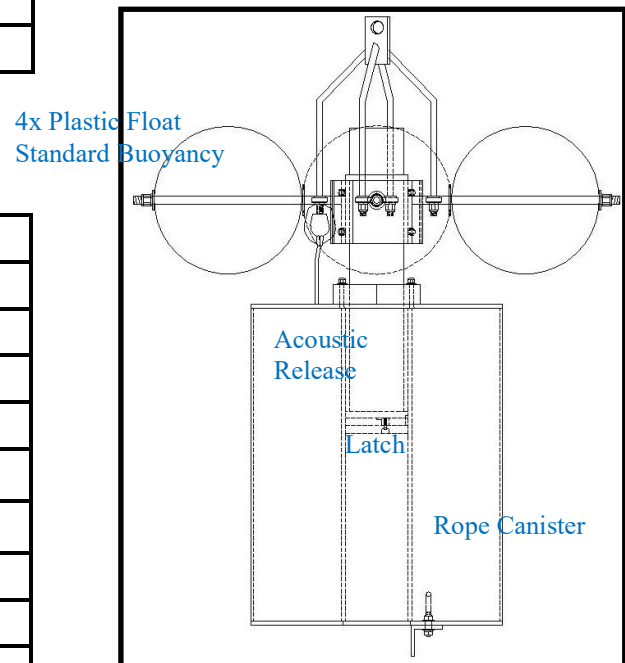
875/500-PUBdeep Assembly Side View
